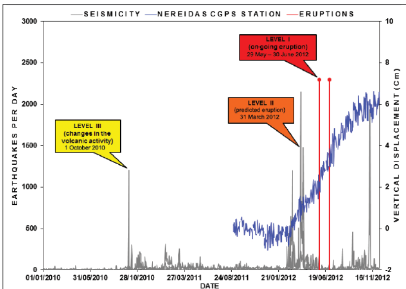
Fig. 2. Vertical deformation (inflation of the volcano's surface) at Nevado del Ruiz, measured at the CGPS site Nereidas (NERE; see Figure 1), is shown in blue. Deformation is compared to seismicity (gray lines) and alert levels issued by the Manizales Volcano Observatory and government officials. Seismic data are critical for the monitoring of Nevado del Ruiz, and the alerts correspond to spikes in seismic activity and release of volcanic gases.
